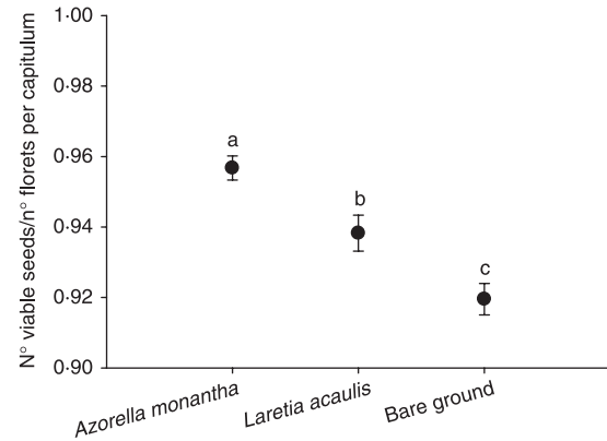
Fig. 6. Reproductive output of Taraxacum officinale individuals growing within cushions of Azorella monantha , Laretia acaulis and open areas outside cushions (bare ground) at 3200 m elevation in the Andes of central Chile. Error bars indicate 2 SE. Different letters indicate significant differences ( t -test, P < 0.05 ).
