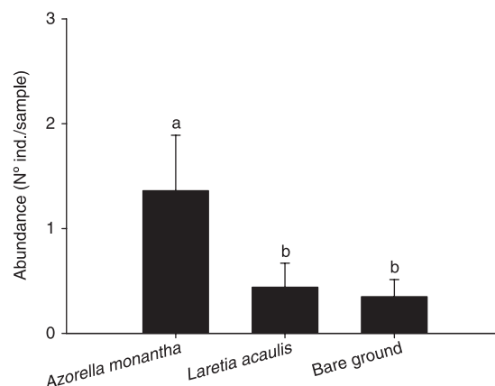
Fig. 3. Abundance of Taraxacum officinale within cushions of Azorella monantha , Laretia acaulis and bare ground at 3200 m in the Andes of central Chile. Error bars indicate 2 SE. Different letters indicate significant differences ( t -test, P < 0.05 ).
