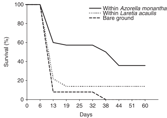
Fig. 4. Kaplan–Meyer estimation of survival of experimentally planted seedlings of Taraxacum officinale within cushions of Azorella monantha , Laretia acaulis and bare ground points at 3200 m elevation in the Andes of central Chile.
