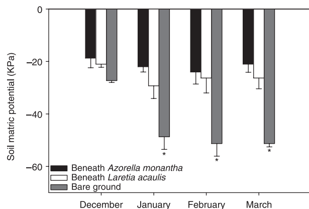
Fig. 2. Soil matric potential within cushions of Azorella monantha , Laretia acaulis and bare ground points during the growing season at 3200 m elevation in the Andes of central Chile. Error bars indicate 2 SE. Asterisks indicate significant differences (Tukey's HSD, P < 0.05 ).
