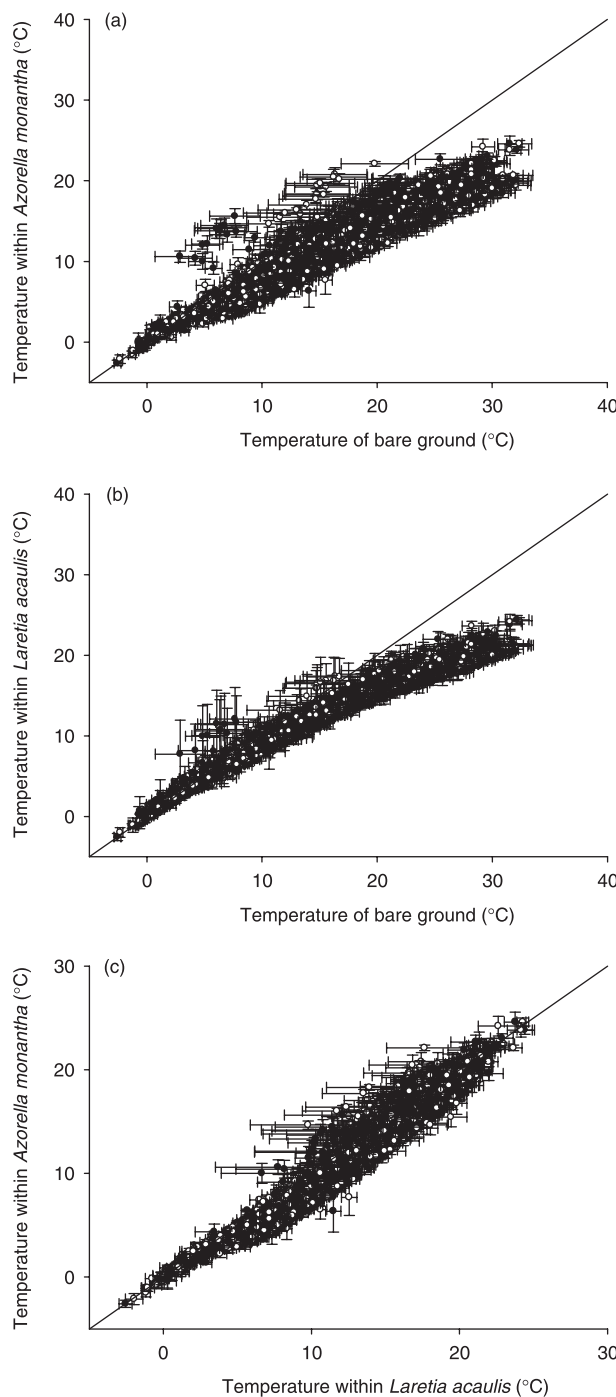
Fig. 1. Substrate temperatures simultaneously registered during the entire growing season within cushions of Azorella monantha and bare ground points (a), within cushions of Laretia acaulis and bare ground points (b), and within the two cushion species (c) at 3200 m elevation in the Andes of central Chile. Error bars indicate 2 SE.
