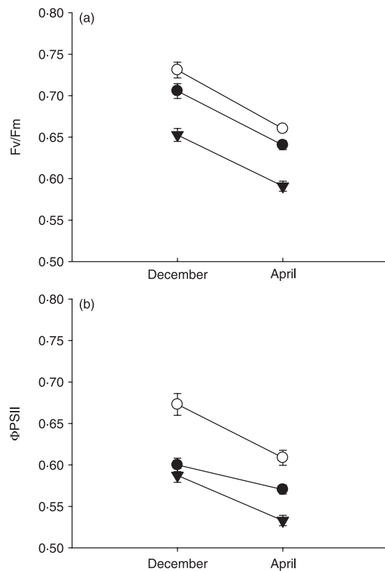
Fig. 5. Chlorophyll fluorescence (Fv/Fm) (a) and photochemical efficiency of photosystem II (ΦPSII) (b) of Taraxacum officinale individuals growing within Azorella monantha cushions (○), within Laretia acaulis cushions (●), and outside cushions (▼) at 3200 m elevation in early (December) and late (April) periods of the growing season in the Andes of central Chile. Error bars indicate 2 SE.
